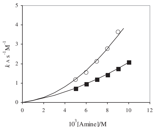
Figure 1. Second-order rate coefficients, k_A , for the reactions of 2,4-dinitrofluorobenzene (DNFB) with (○) 3-dimethylamino-1-propylamine (DMPA) and (■) ethylenediamine (EDA) in toluene at 25.0 \pm 0.2 °C as a function of amine concentration
