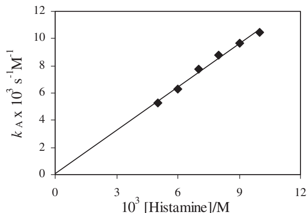
Figure 5. Second-order rate coefficients, k_A , for the reactions of 2,4-dinitrofluorobenzene (DNFB) with histamine in toluene at 40.0 \pm 0.2^\circ\text{C} as a function of histamine concentration
