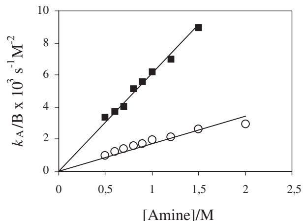
Figure 4. Third-order rate coefficients, k_A/[B] , for the reactions of 2,4-dinitrochlorobenzene (DNCIB) with (○) 3-dimethylamino-1-propylamine (DMPA) and (■) ethylenediamine (EDA) in toluene at 25.0 \pm 0.2^\circ\text{C} as a function of amine concentration
