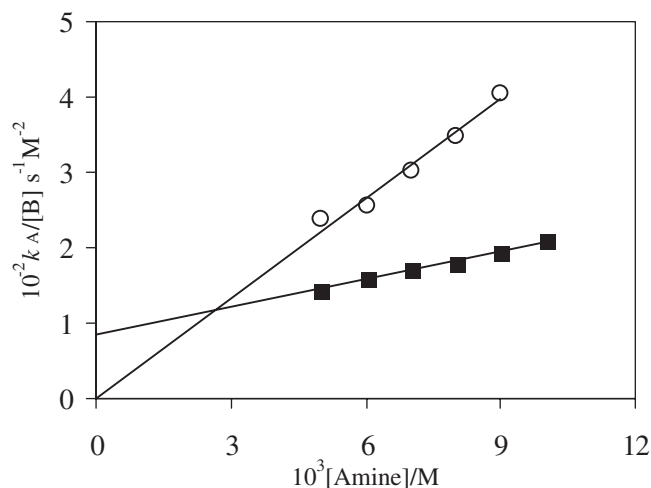
Figure 2. Third-order rate coefficients, k_A/[B] , for the reactions of 2,4-dinitrofluorobenzene (DNFB) with (○) 3-dimethylamino-1-propylamine (DMPA) and (■) ethylenediamine (EDA) in toluene at 25.0 \pm 0.2 °C as a function of amine concentration
