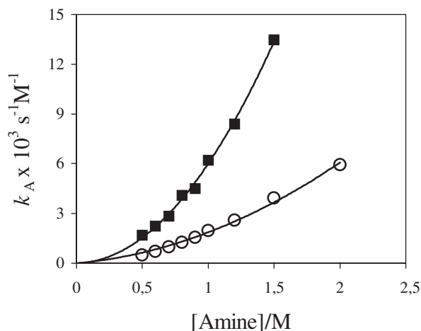
Figure 3. Second-order rate coefficients, k_A , for the reactions of 2,4-dinitrochlorobenzene (DNCIB) with (○) 3-dimethylamino-1-propylamine (DMPA) and (■) ethylenediamine (EDA) in toluene at 25.0 \pm 0.2^\circ\text{C} as a function of amine concentration
